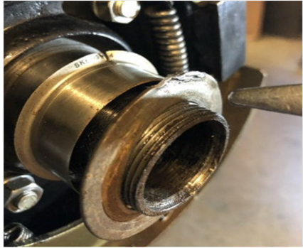
Sleeve on other side being fitted using an old locking Washer to gently ease it over the axle.
