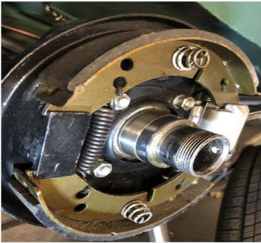
Here sleeve incorrectly fitted too far back Also note slight damage still exposed.
